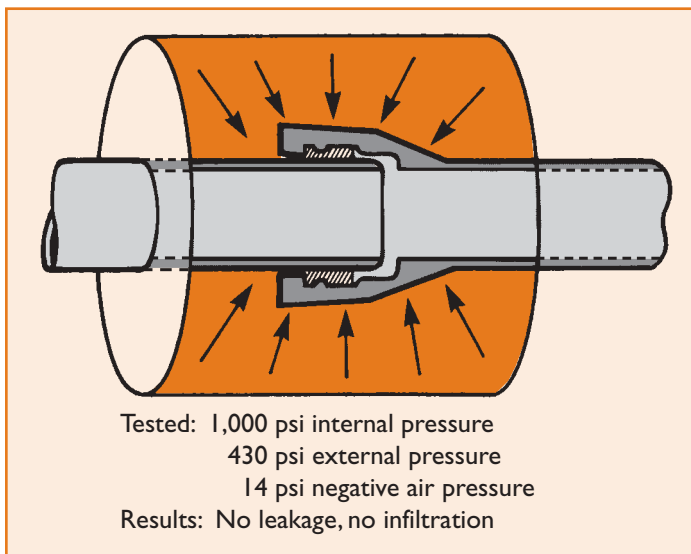
Figure 2: Ductile Iron Push-on Joint Test
