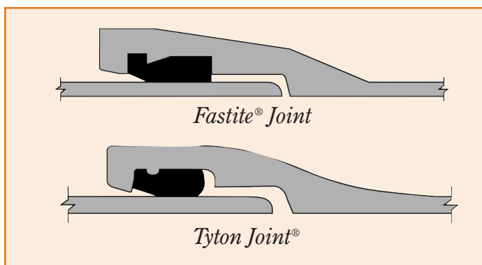
Figure 3: Ductile Iron Push-on Joints
